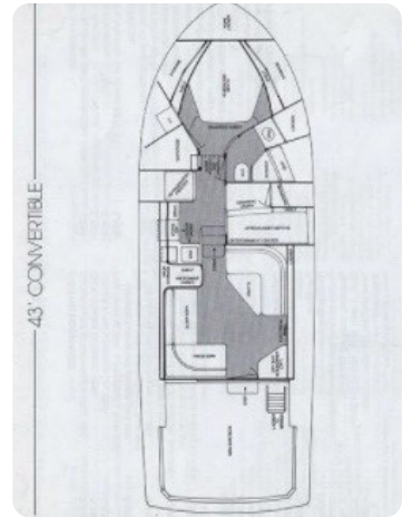
Bertram 43 Conv layout
