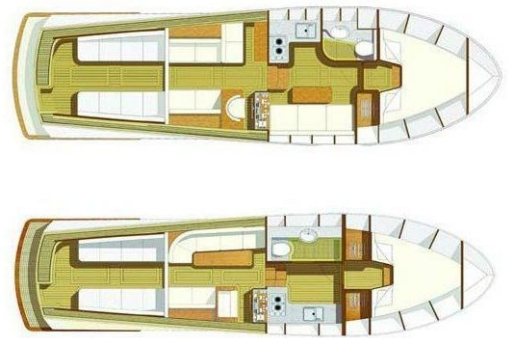
Liberty 35 Layout
