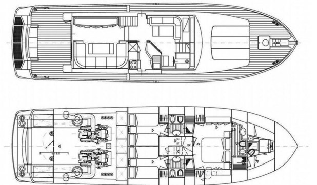
SANLORENZO SL 62 layout
