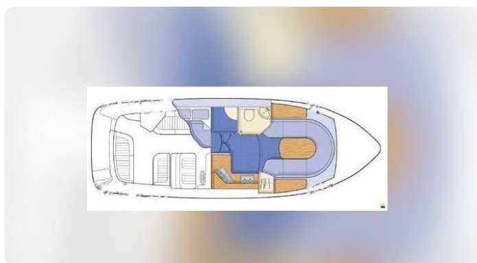
Layout Sealine 28 Sport
