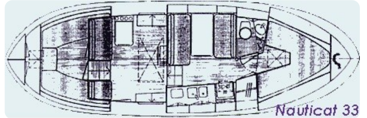
Nauticat 33 _ Layout
